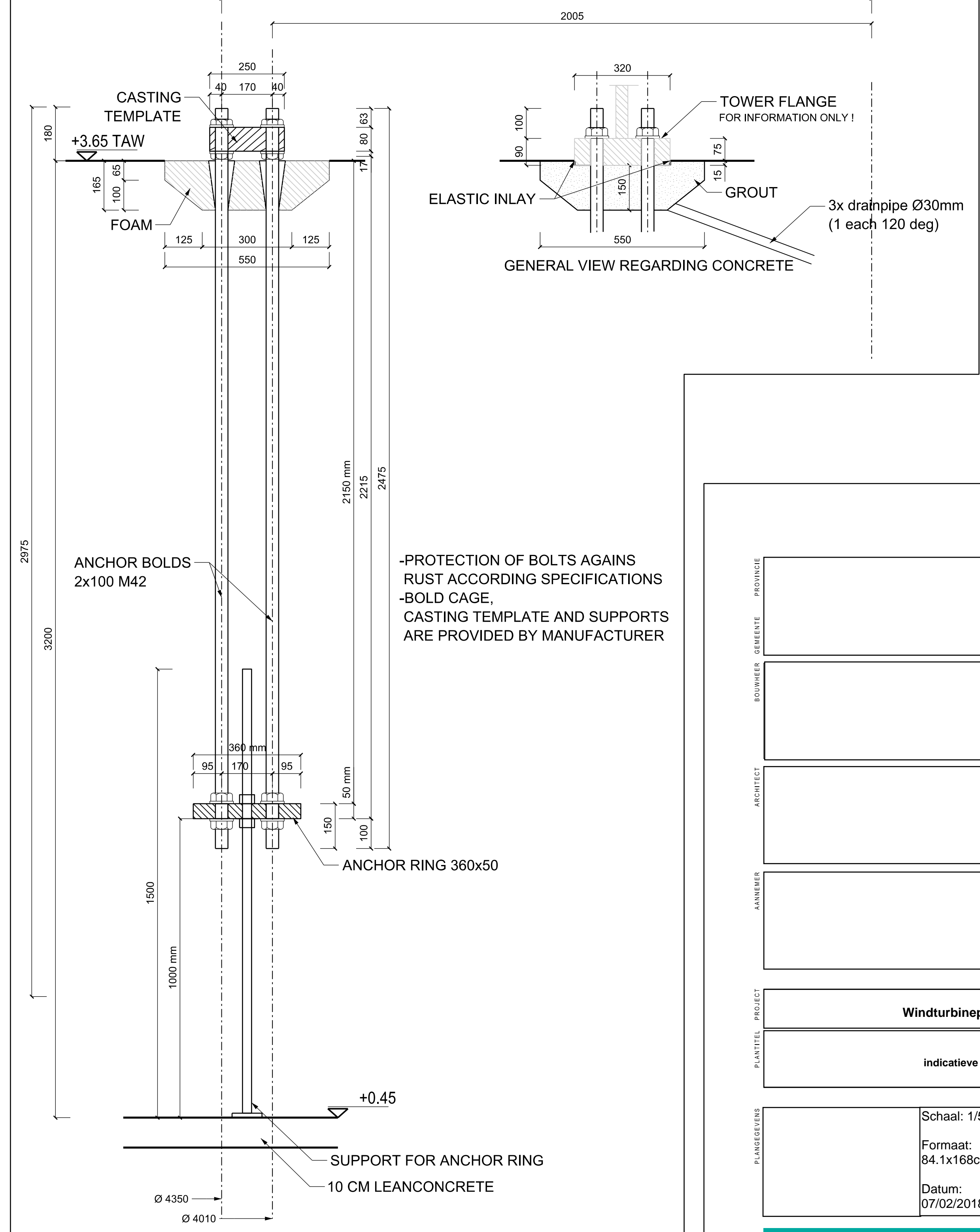
DETAILS ANCHOR CAGE SCALE: 1/10
