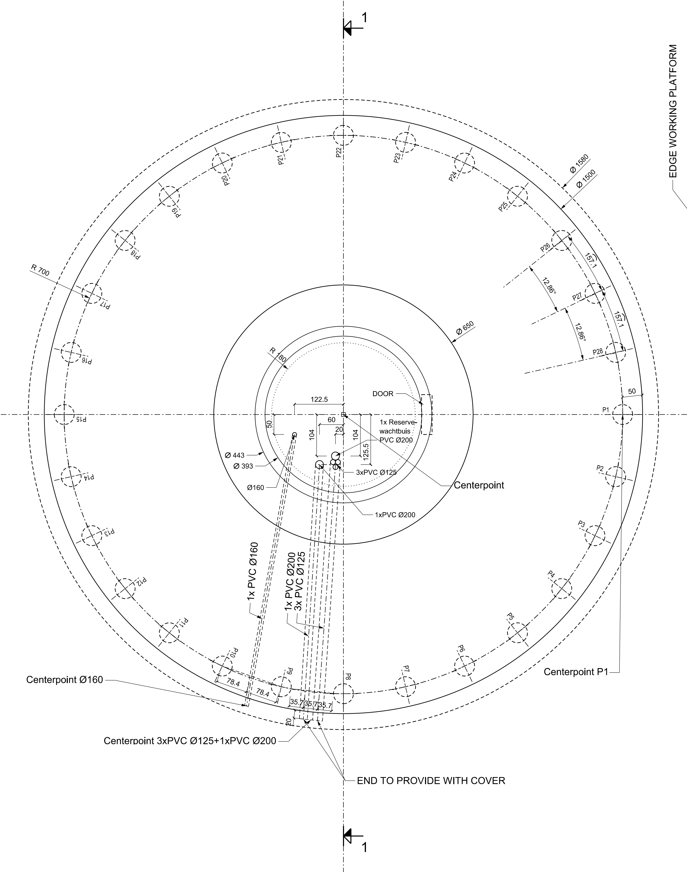
PLAN VIEW WT1 SCALE: 1/50
