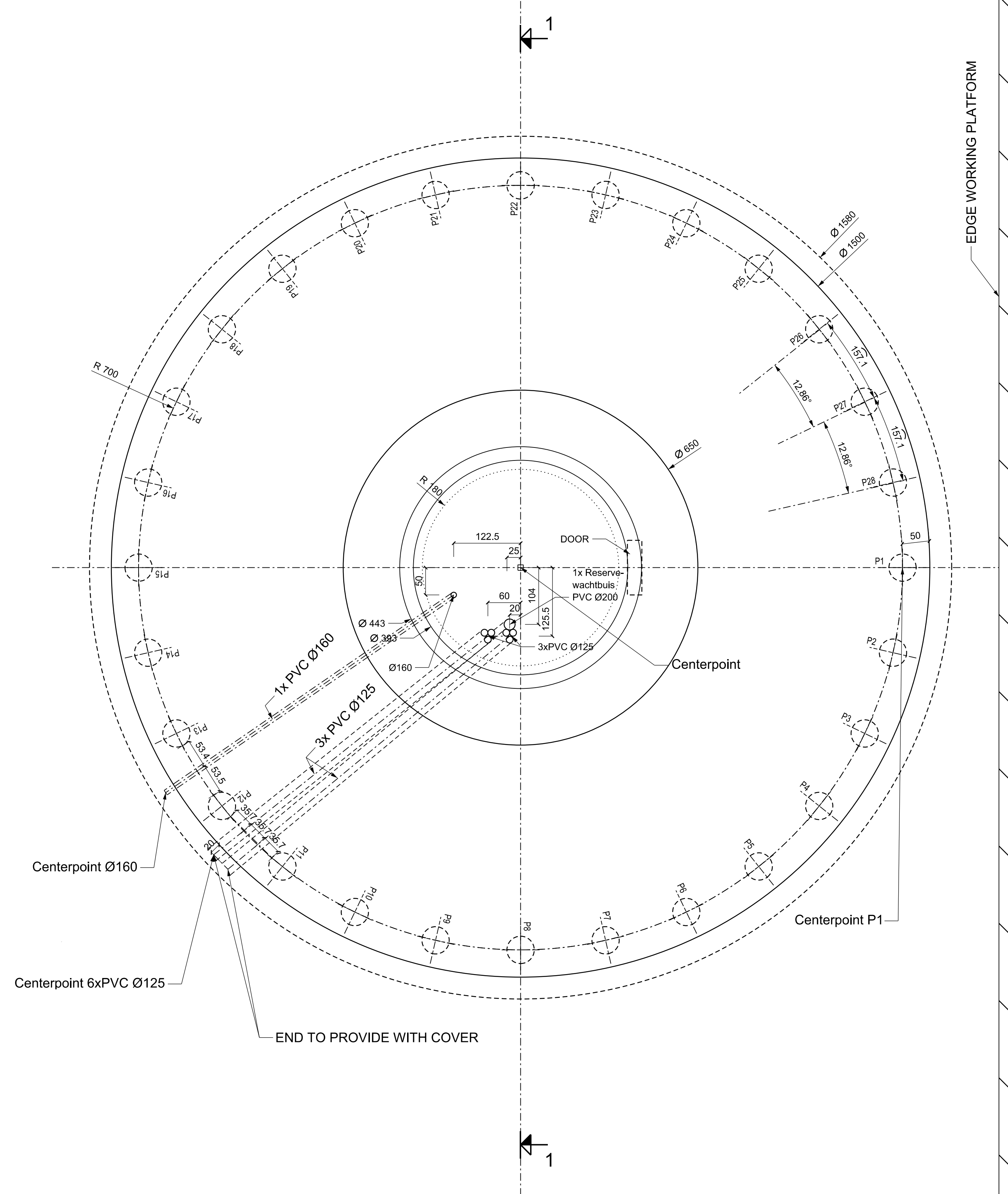
PLAN VIEW WT2 SCALE: 1/50
